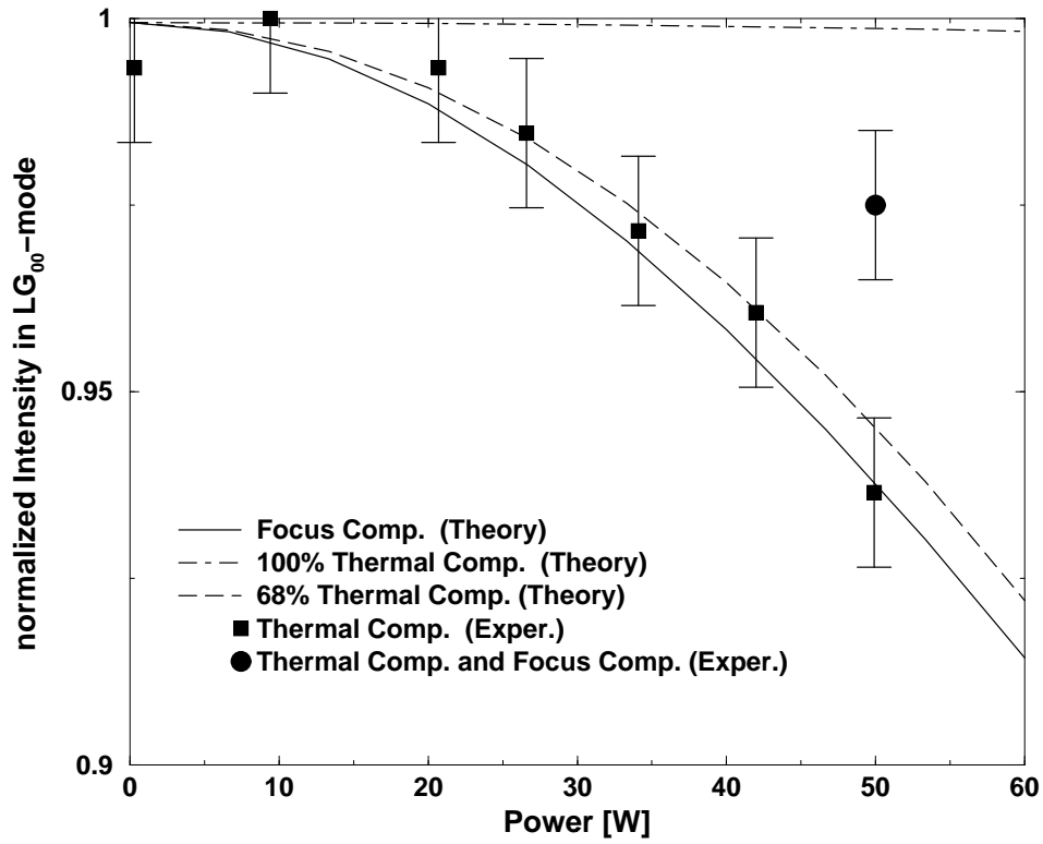
Figure 3. The intensity in the fundamental cavity eigenmode normalized to the intensity at 0 W pump power, except for the thermal compensated experimental data, where we used the larger value at 9 W pump power. The difference between the two data points is within the error bars of the experiment. The solid line shows the focus compensated case. The dot dashed line shows the intensity for matched (100%) compensation, while the dashed line shows the intensity for the case where the compensator crystal has only 68% of the optimum length. The experimental data (squares) could be explained by focus compensation or 68% thermal compensation. As we were able to increase the intensity in the fundamental mode of the cavity by changing the mode matching (circle) it is obvious that we were not focus compensated.
